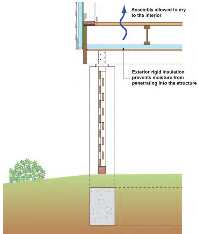
Figure 18: Foundation Vapor Management
