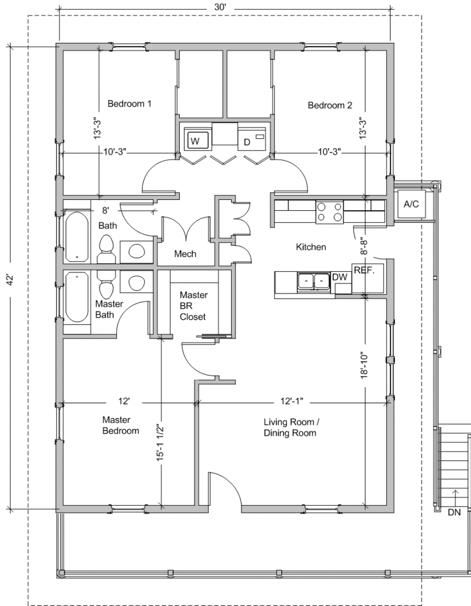
Figure 2: Hot-Humid Climate house floor plan
