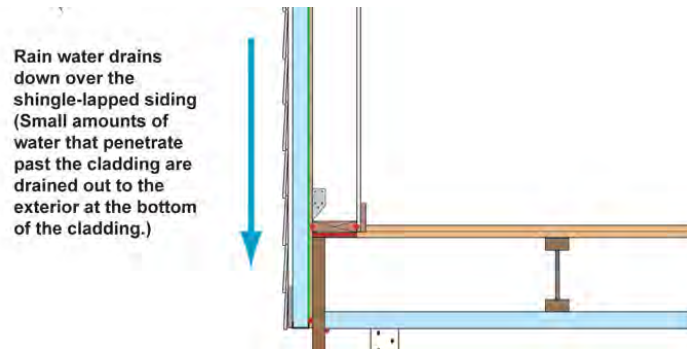
Figure 12: Wall Drainage
