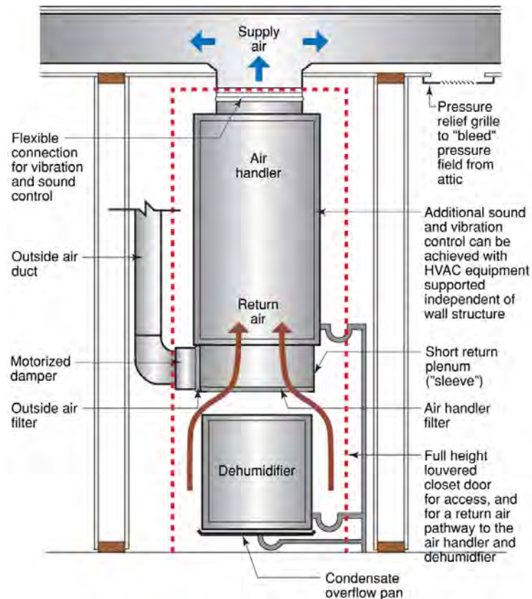
Figure 24: Air Handler Schematic
