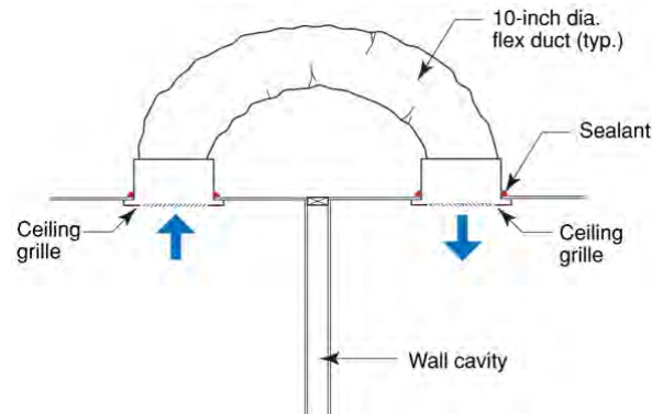
Figure 27: "Jump Duct" over interior partition wall
