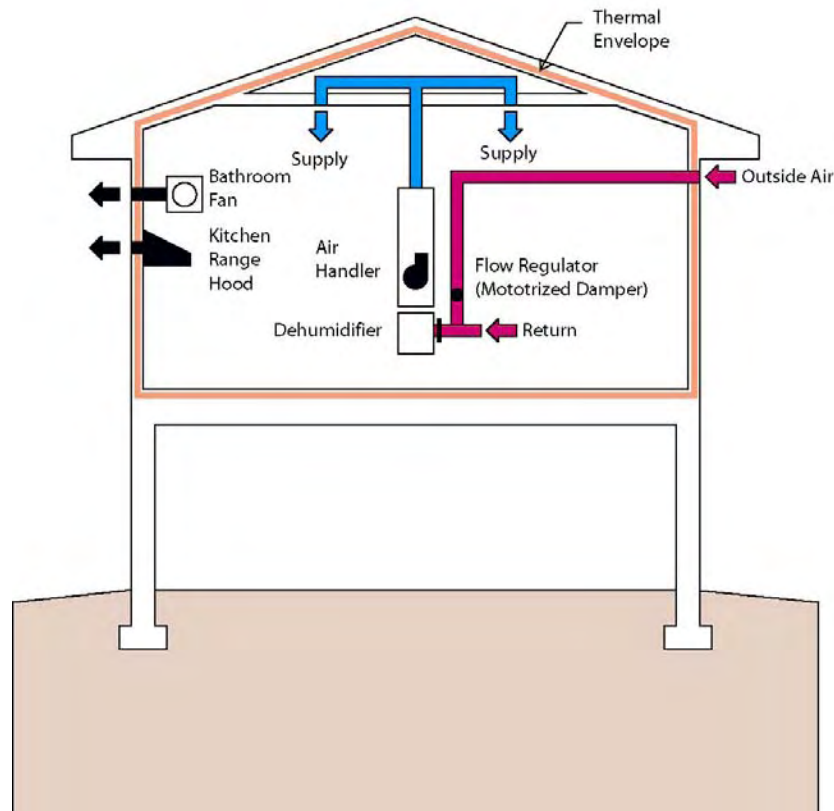
Figure 22: Mechanical Schematic for Hot Humid House
