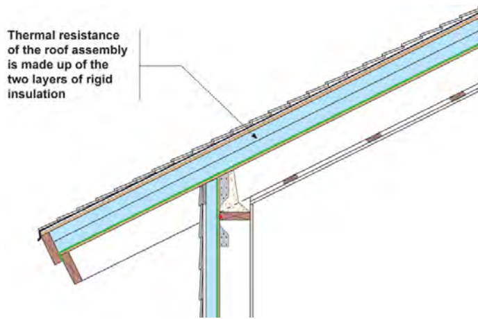
Figure 11: Roof Thermal Resistance
