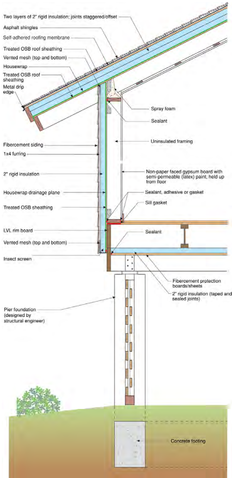
Figure 5: Building Section
