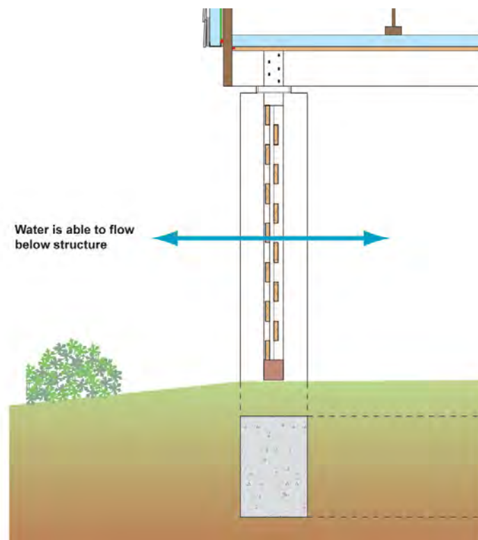
Figure 16: Foundation Drainage
