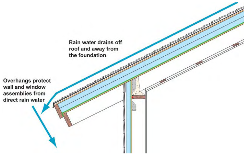
Figure 8: Roof Drainage
