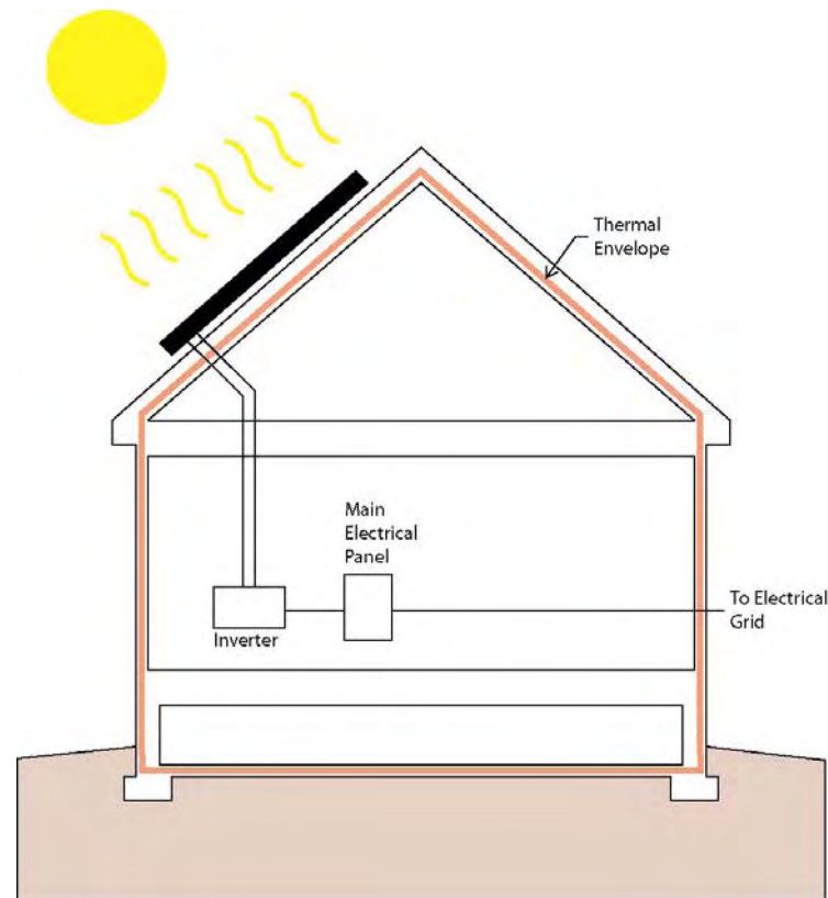
Figure 32: Schematic of a Photovoltaic System Design Considerations
