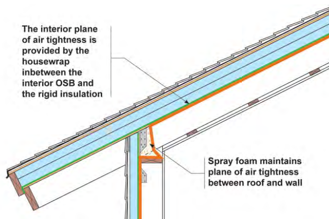
Figure 9: Roof Air Barrier
