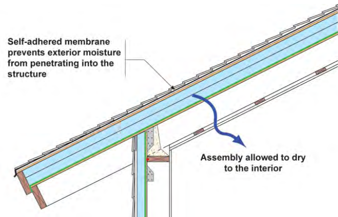
Figure 10: Roof Vapor Management
