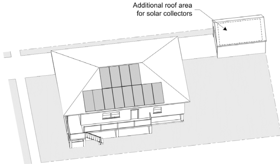
Figure 33: Arrangement of Photovoltaic Array on ZEH
