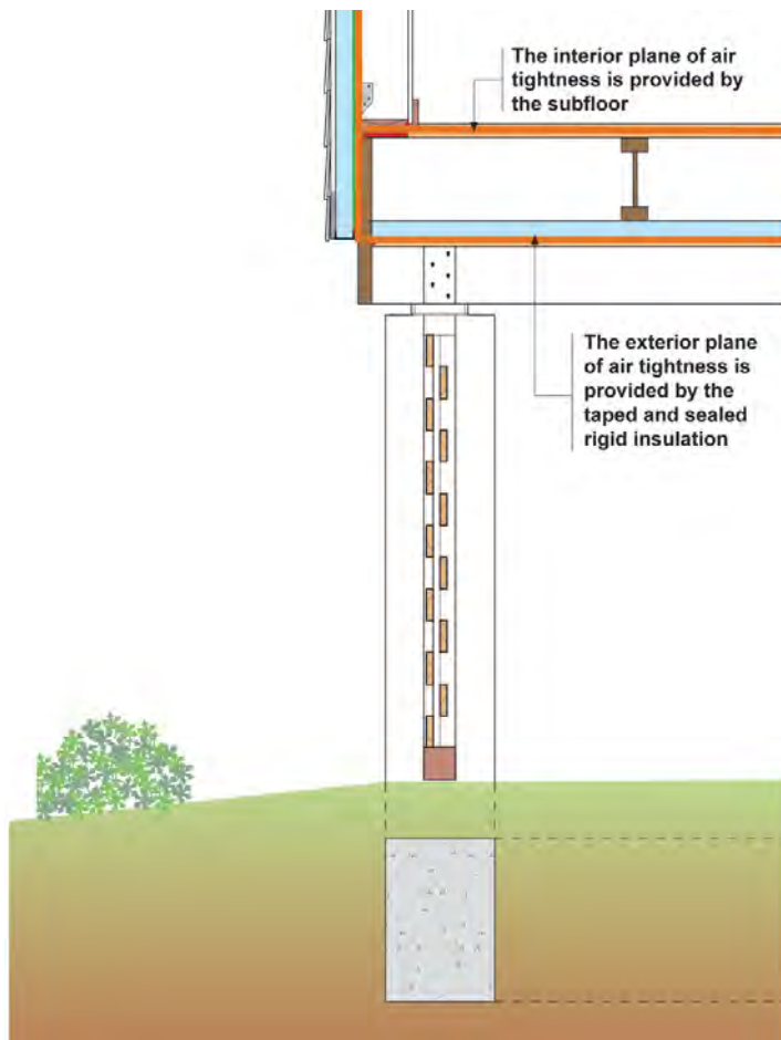
Figure 17: Foundation Air Barrier
