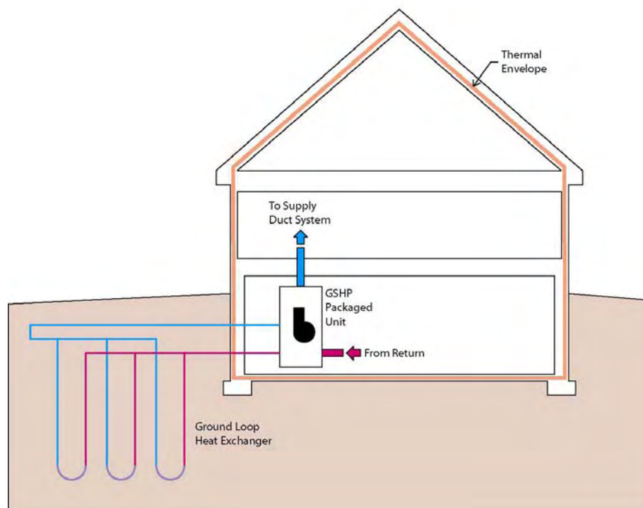
Figure 30: Schematic of a Ground Source Heat Pump
