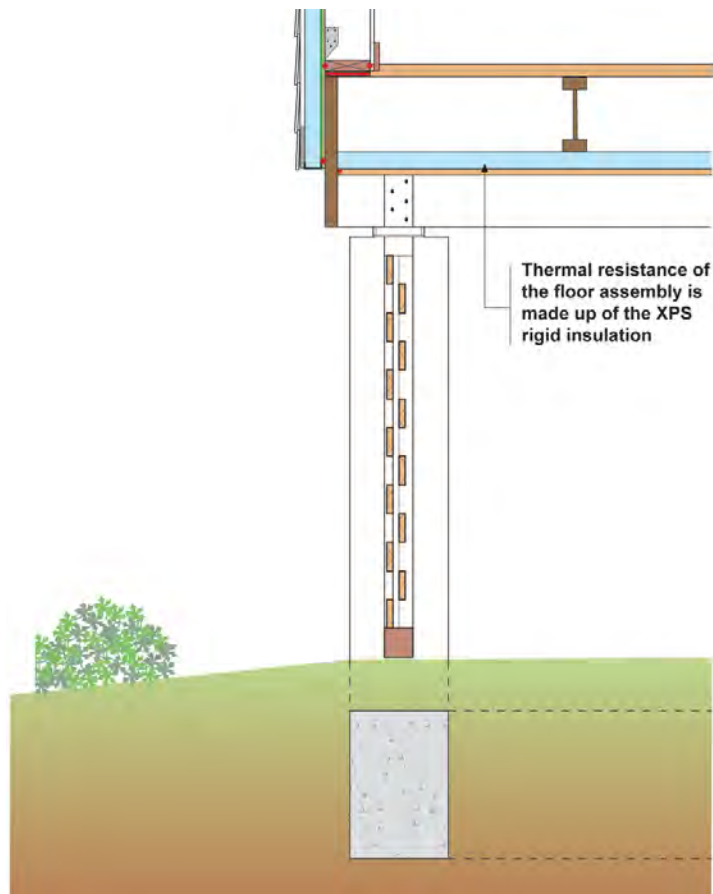
Figure 19: Foundation Thermal Resistance
