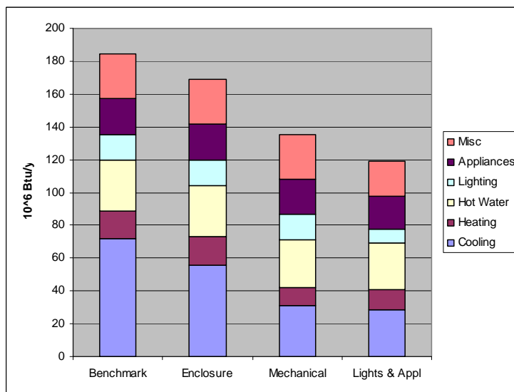
Figure 4: Total Source Energy Consumption Reduction
